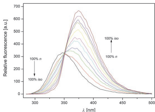
Figure 1. Fluorescence spectra of 5a and 6a and their mixtures ( 5a:6a =10:0, 9:1, ..., 1:9, 0:10) in DMSO, \lambda_{\text{ex}} =275 nm, c =20 \mu\text{M} at 25 °C.
