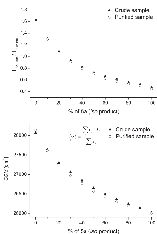
Figure 2. Regioselectivity profiles of both crude and pure 5a and 6a and their mixtures in DMSO, \lambda_{\text{ex}} =275 nm, c =20 \mu\text{M} at 25 °C.
