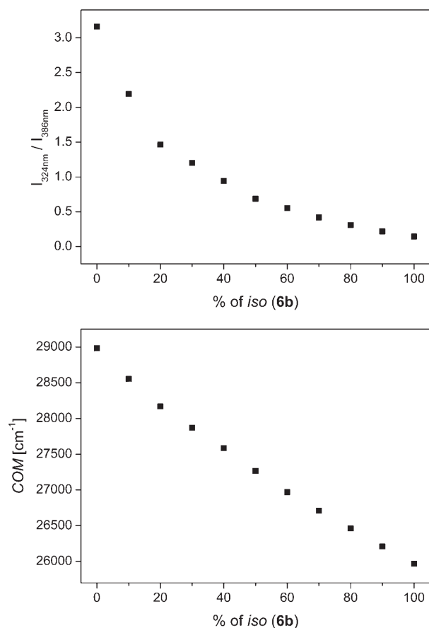
Figure 4. Ratio of the fluorescence intensity at the two emission maxima (of n - and iso -regioisomer, respectively) (top) and COM of the emission spectra (bottom) vs. the molar ratio of the two regioisomers of 5b/6b pair at \lambda_{\text{ex}}=275 nm.
