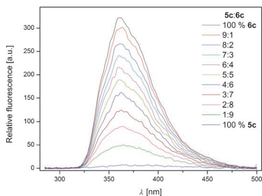
Figure 5. Fluorescence spectra of 5c , 6c and their mixtures ( \lambda_{\text{ex}}=275 nm, DMSO, c=20 \mu\text{M} , 25^\circ\text{C} ).
