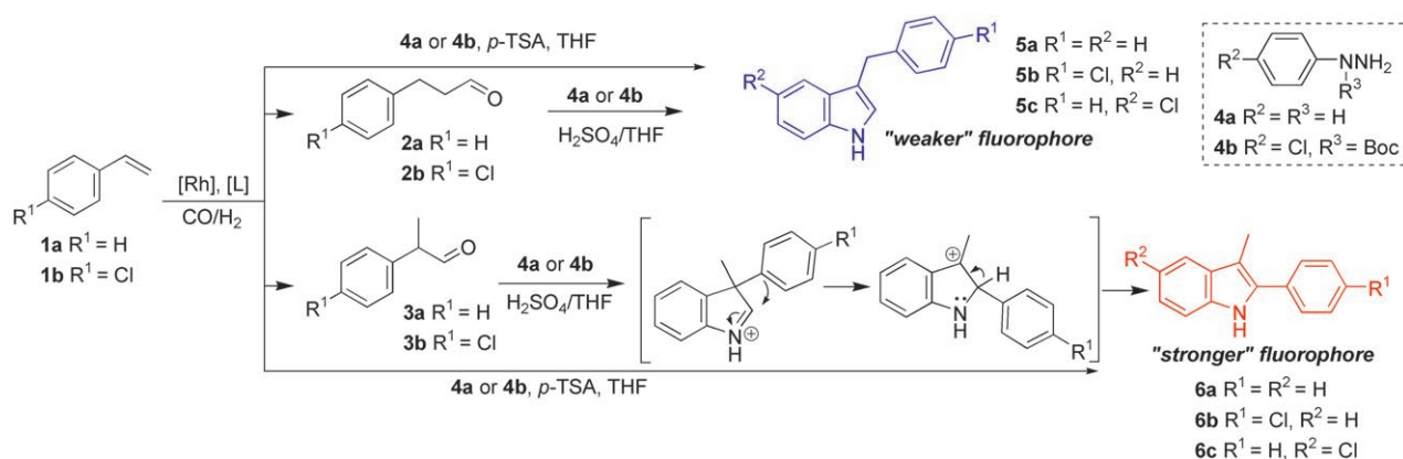
Scheme 1. Synthesis of indoles via tandem or stepwise hydroformylation/Fischer-indolization.
