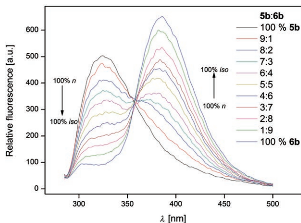
Figure 3. Fluorescence spectra of 5b , 6b and their mixtures ( \lambda_{\text{ex}} =275 nm, DMSO, c =5 \mu\text{M} , 25 °C).
