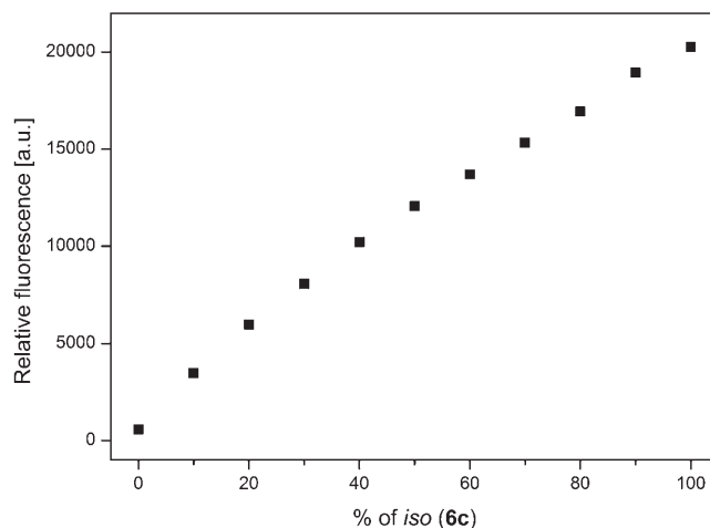
Figure 6. Maximum emission intensity ( \lambda_{\text{em}}=361 nm) vs. ratio of the regioisomers ( \lambda_{\text{ex}}=275 nm) of the 5c/6c pair.
